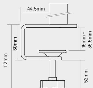
C-clamp
