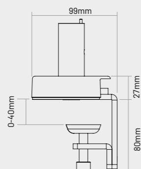
Split C-clamp
